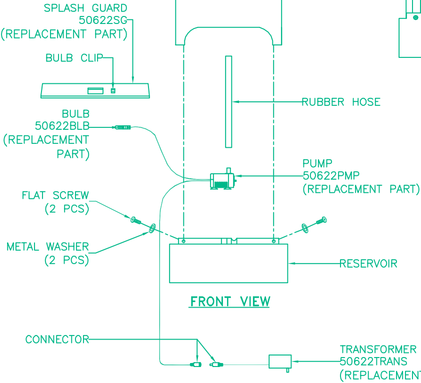
FOUNTAIN ASSEMBLED VIEW:
